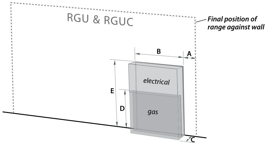
Fig. 11 Location of electrical and gas supply - RGU & RGUC models
