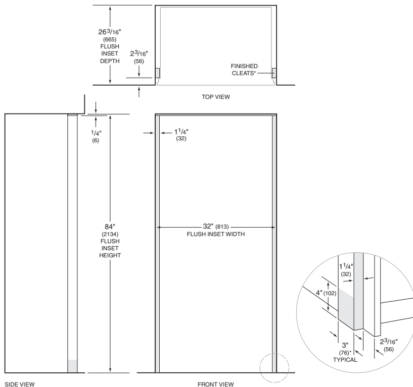
*3" (76) typical depth. Shaded areas will be visible and should be finished to match cabinetry. NOTE: Shaded line represents profile of unit with 3/4" (19) panel.
