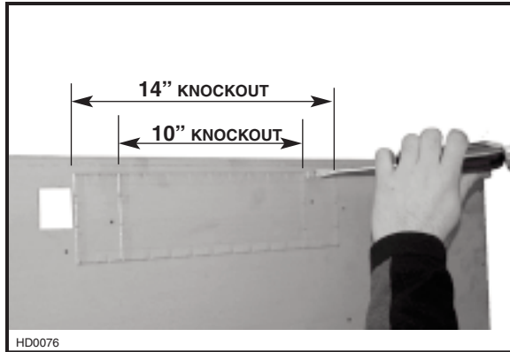
HD0076 Removing horizontal knockout opening on back of hood
