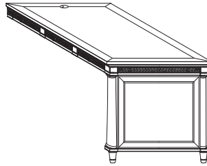
I88-344 Partner's Desk Top and End Panel 60W x 31H x 32D
