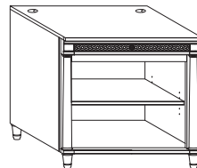
I88-345 Partner's Desk Base 32W x 31H x 25D
