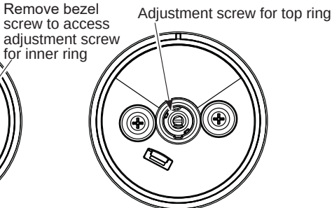
Adjustment screw for dual-flame stacked burner top ring of flames only (no adjustment for bottom ring)
