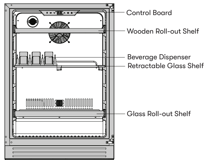
PRPB24C01CG without door and with beverage dispenser and retractable glass shelf
