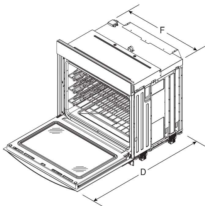
ANGLED VIEW
