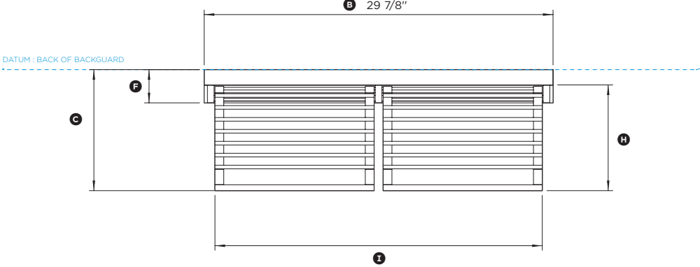
PLAN VIEW
