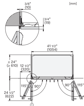
KFMC3858FD, MasterCool III, PACS, with stainless steel front, top view (US)
