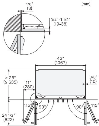
KFMC3858FD, MasterCool III, top view, panel ready (US)
