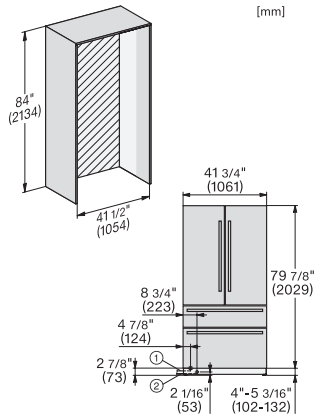
KFMC3858FD, MasterCool III, PACS, with stainless steel front, installation (US)
