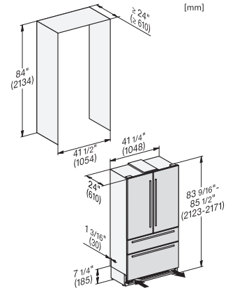
KFMC3858FD, MasterCool III, PACS, with stainless steel front, integration (US)
