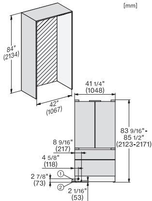
KFMC3858FD, MasterCool III, installation, panel ready (US)
