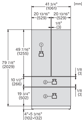
KFMC3858FD, MasterCool III, front view (US)
