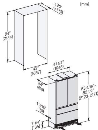
KFMC3858FD, MasterCool III, integration, panel ready (US)
