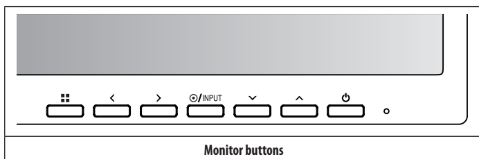
[Quick Settings]
