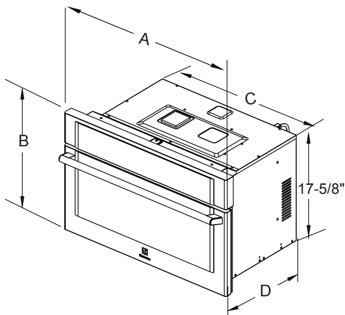
Figure 2: Micro-ondes uniquement
