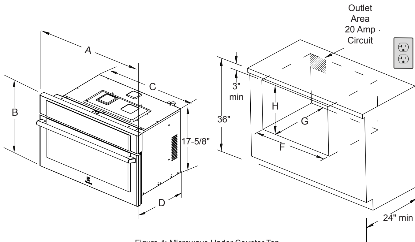
Figure 4: Microwave Under Counter Top
