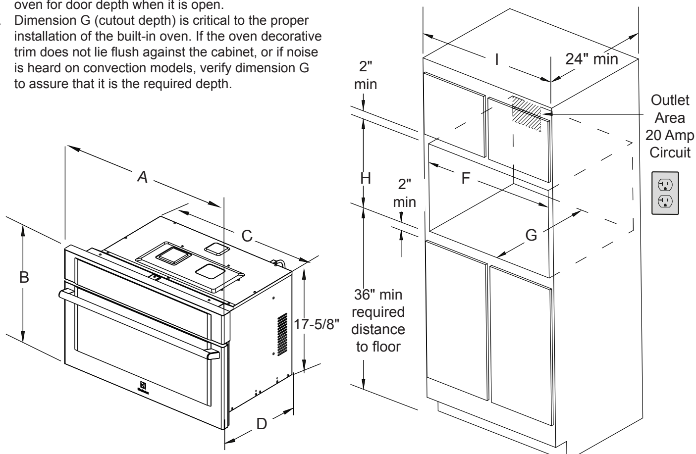
Figure 2: Microwave Only
