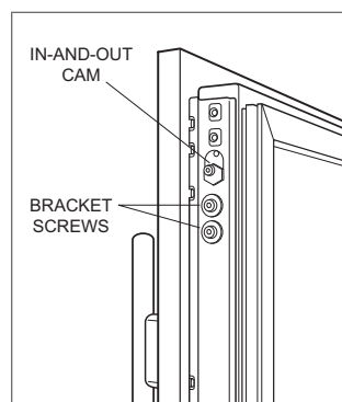
In-and-out adjustment
