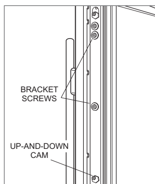
Up-and-down adjustment
