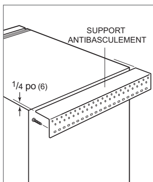
Support antibasculement
