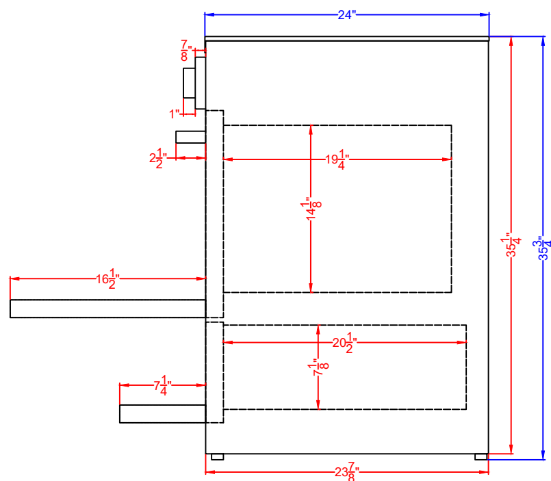
Profile View
