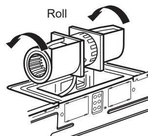
AFTER: Fan Blade Openings Facing Forward
