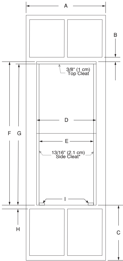
FRONT VIEW
