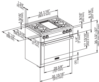
HR1936G, HR1936-2, HR1936-3 (installation drawing)
