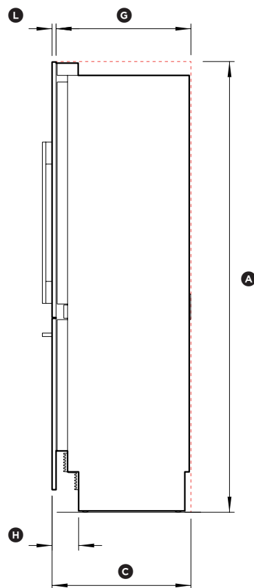
PROFILE VIEW
