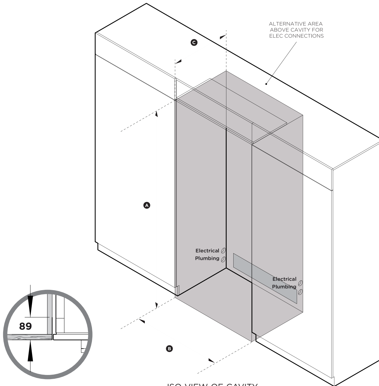
Frameless: Finished return, sides and top
