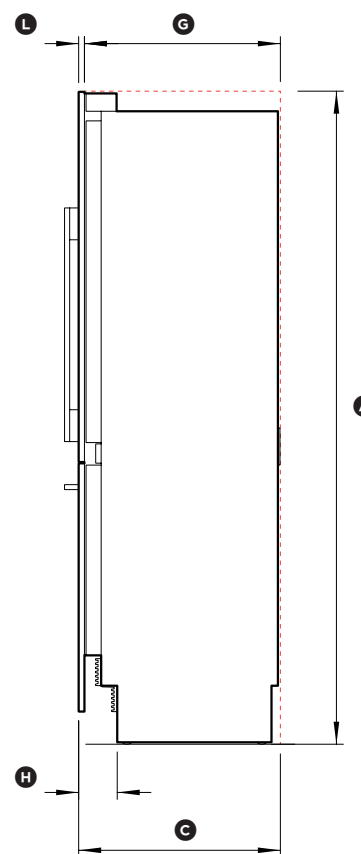
PROFILE VIEW
