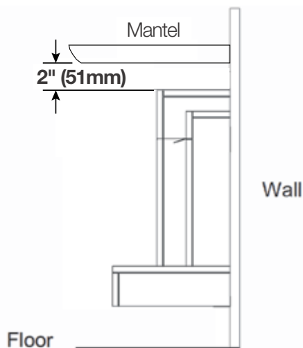
Side View (Wall Mount) NEFP32-5019W Illustrated
