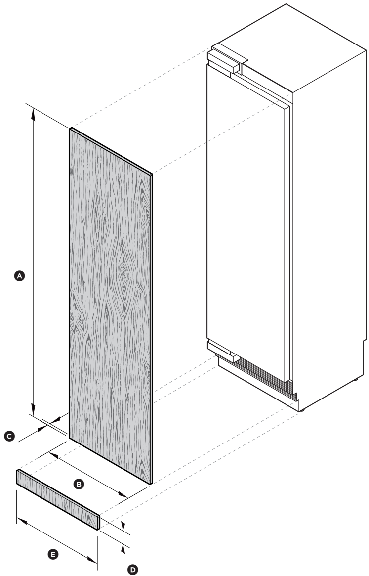
ISO VIEW
