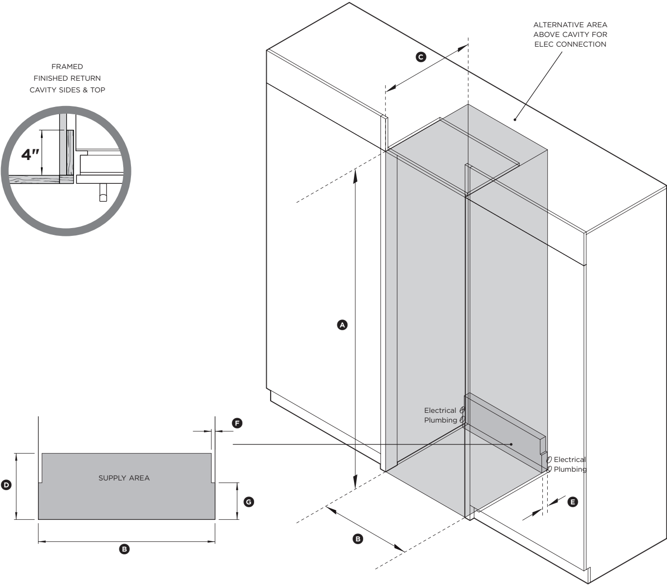
ISO VIEW OF CAVITY
