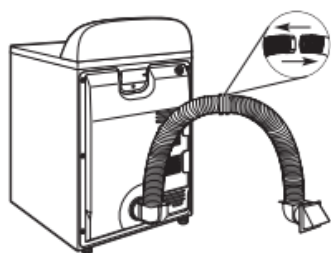
Over-The-Top installation (also available with one offset elbow). Semi rigid venting used in this example.
