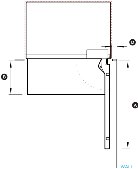
90° DOOR OPENING
