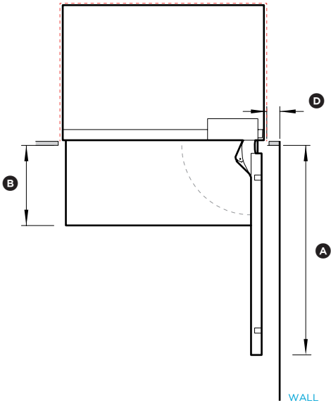
90° DOOR OPENING
