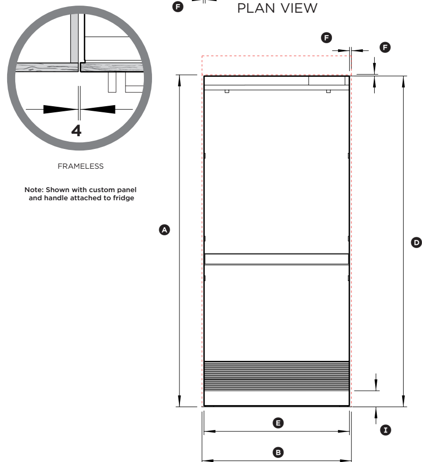
FRONT VIEW
