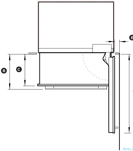
90° DOOR OPENING
