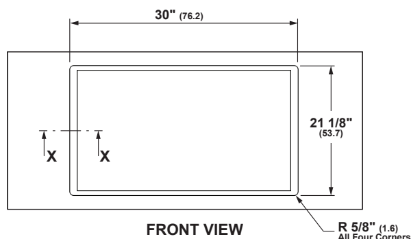
TOP VIEW OF CUTOUT
