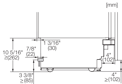
Side-by-side, MasterCool, without partition wall, with heating mat (Sketch)
