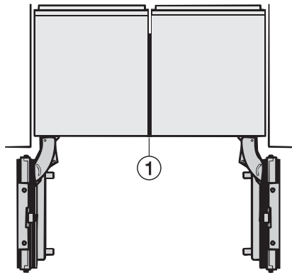
Side-by-side, MasterCool, without partition wall, with heating mat (Sketch)
