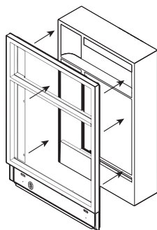
Align Mounting Locations
