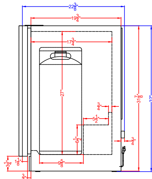
PROFILE VIEW
