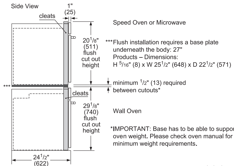
Flush Installation Over Single Oven
