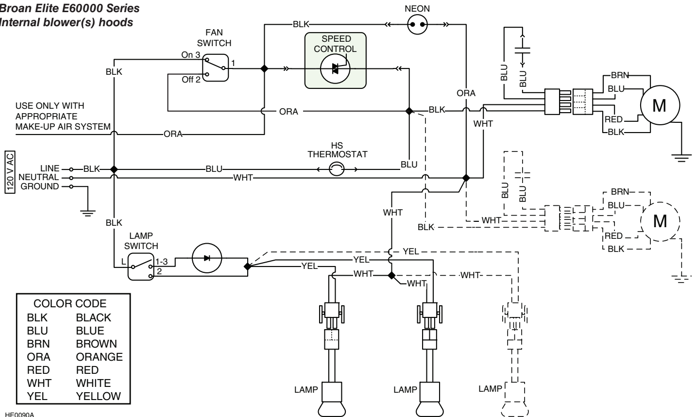
Broan Elite E60000 Series Exterior or In-Line blower hoods
