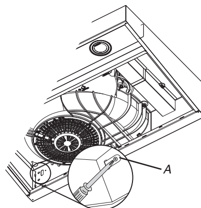
A. #8-18 x \frac{5}{8} " (4.2 x 16 mm) screw
