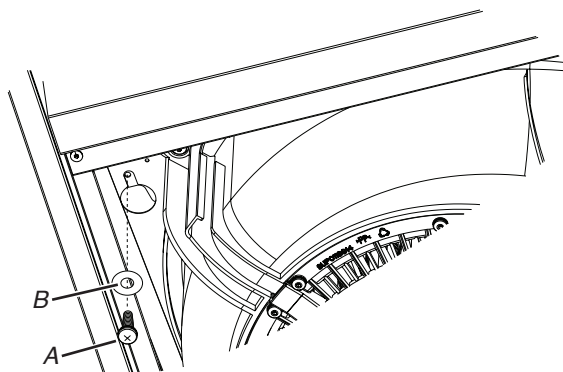
A. #8-18 x \frac{5}{8} " (4.2 x 16 mm) screw B. Washer
