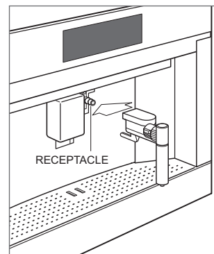
Water spout
