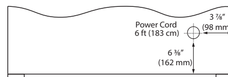
Cabinet Cut-Out
