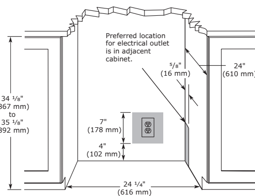
Cabinet Cut-Out
