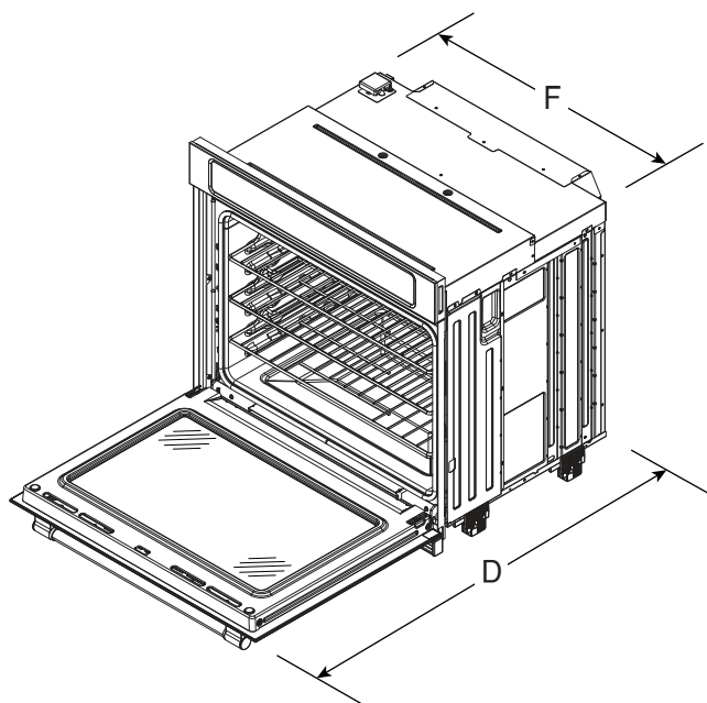
ANGLED VIEW
