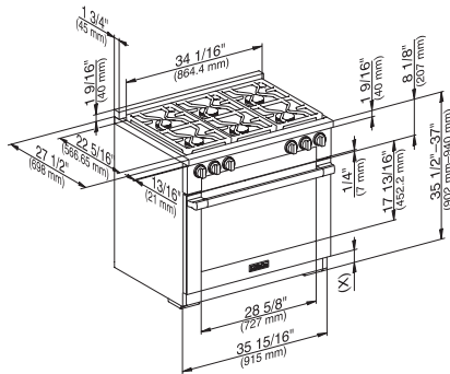
HR1934G, HR1934-2, HR1934-3 (installation drawing)
