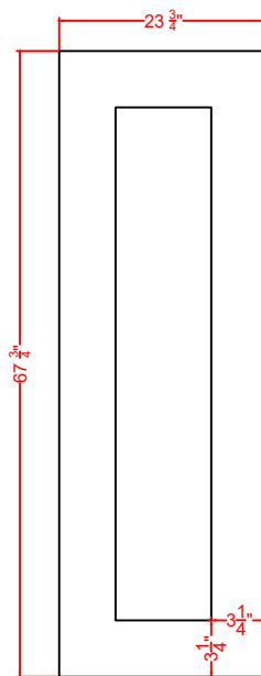
Door Panel Detail
