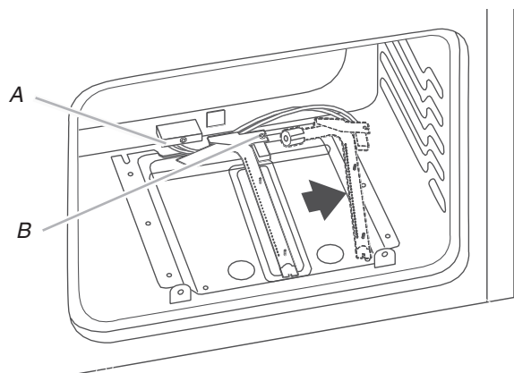
A. Igniter and wires
