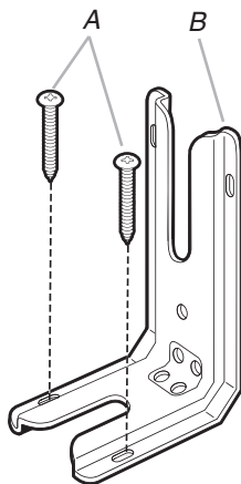
A. #12 x 1 5/8" (4.1 cm) screws B. Anti-tip bracket
