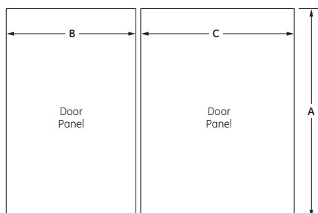
PANEL DIMENSIONS
