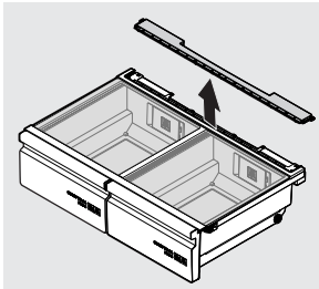
Removing Auto Humidity Control Membrane
