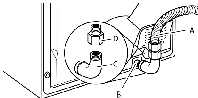
A. 3/8" (9.5 mm) flexible gas connector
