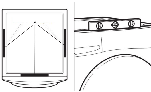
A. Place level here
