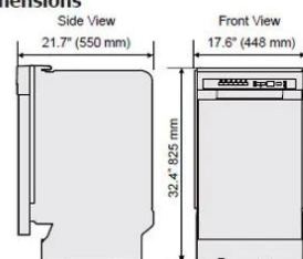
Product dimensions
