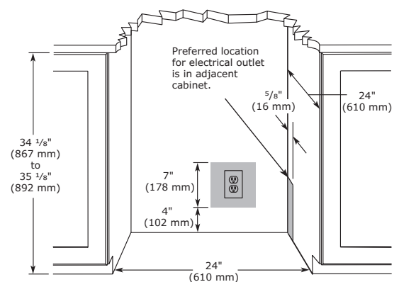
Cabinet Cut-Out
