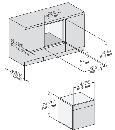
H7x6xBP, Einbau, 30 Zoll, Flush inset, built-under 7/8" – 22" mm – Glas, 15/16" – 23.3" mm – Stainless steel
