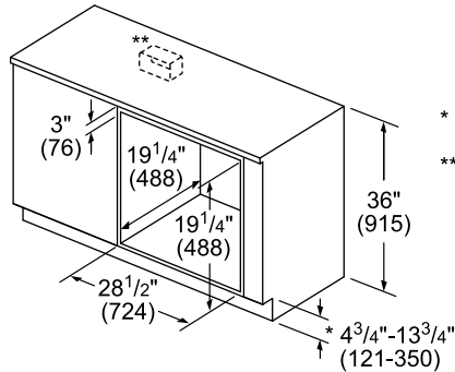
Under-counter Installation
