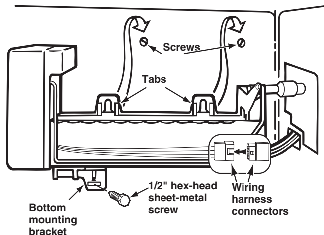
Mounting the ice maker (top and bottom freezers)
