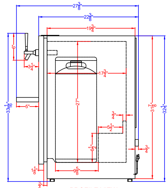
PROFILE VIEW
