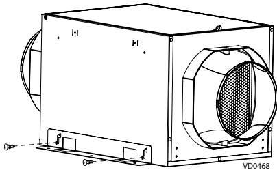
SCREW POSITION ACCORDING TO CEILING THICKNESS
