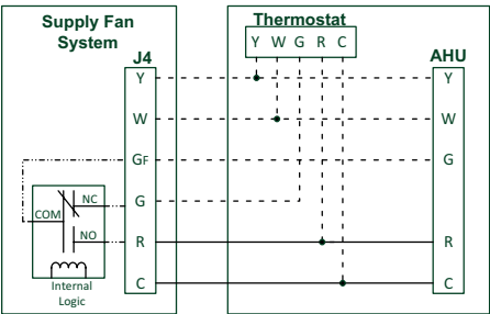
Synchronized: Start AHU blower when supply fan is running
