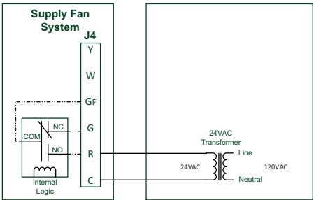
No AHU connection, stand alone supply
