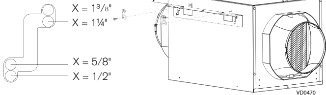
SCREW POSITION ACCORDING TO CEILING THICKNESS
