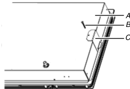
A. Cooktop base bottom B. Attachment screw C. Clamping bracket (end locations recommended)
