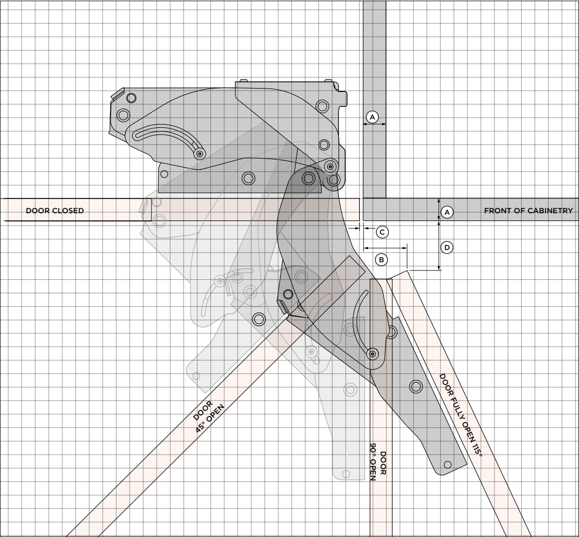
1 SQUARE = 1/2" (12.7mm)
