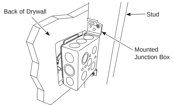
BACK VIEW
