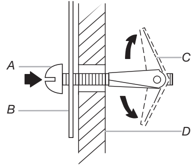
A. \frac{3}{16} -24 x 3" round head bolt B. Mounting plate C. Spring toggle nut D. Drywall
