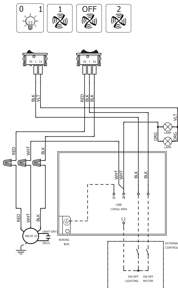
Wiring Diagram 991.0541.846
