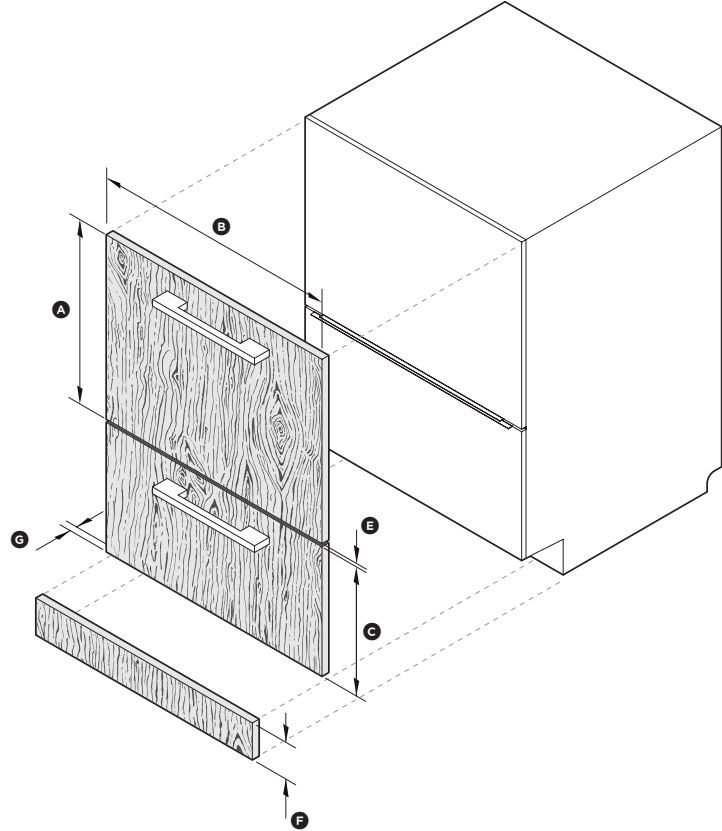
ISO VIEW
